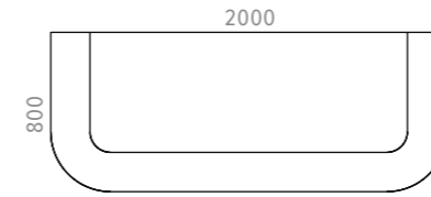
Desktop: 1960 x 780 x H740 mm
