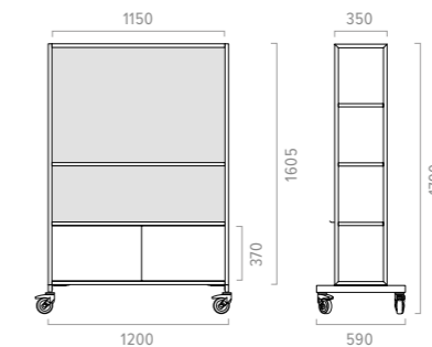
Mobile media wall with fixed shelf + cabinet + back panel
